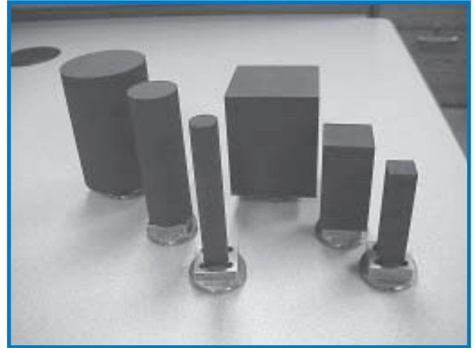
Pre-mounted graphite blanks on EROWA ITS Compact Holders
