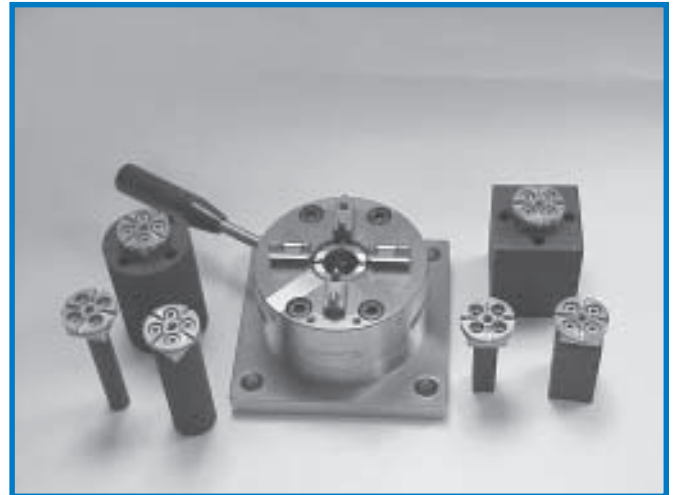
Pre-mounted graphite blanks shown with EROWA chuck
